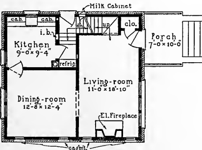
First-floor Plan
